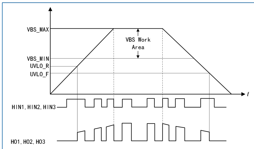
Figure 4-9 High-side Power Supply VBS and Under-voltage Lockout
