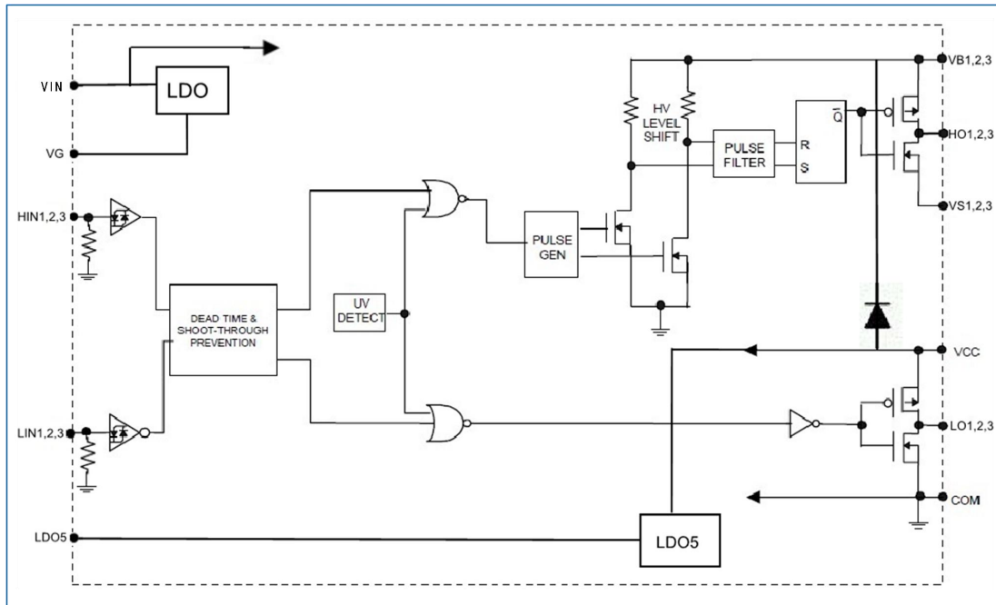
Figure 4-7 Driver Functional Block Diagram
