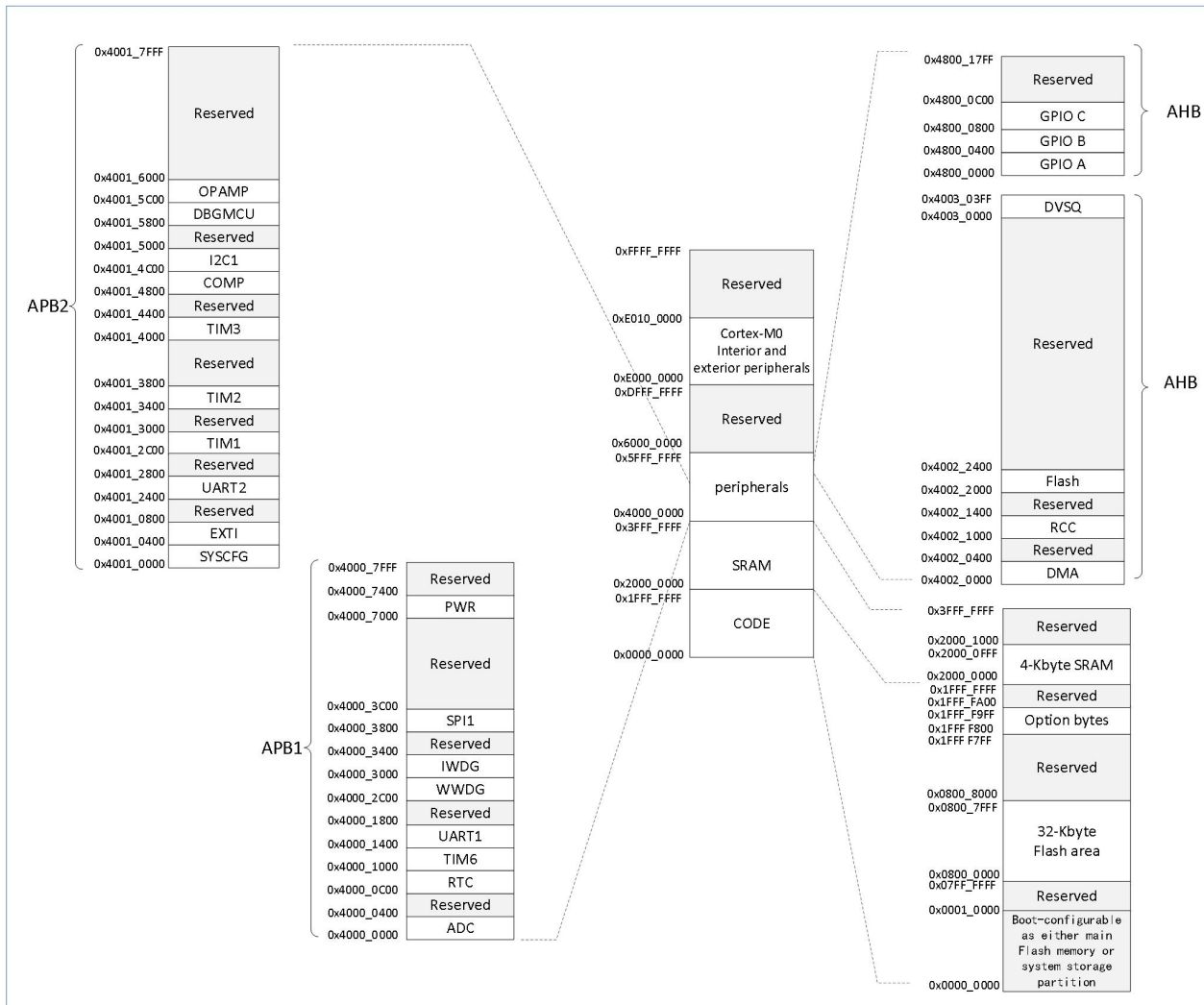
Figure 4-3 PM20025G-08 Memory Mapping
