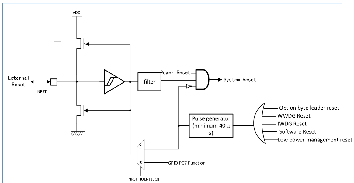
Figure 4-4 Reset Signal
