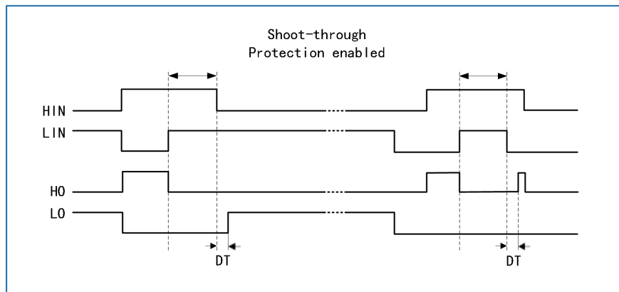
Figure 4-10 Shoot-Through Prevention
