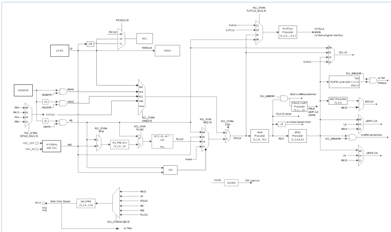
Figure 4-5 Clock Tree
