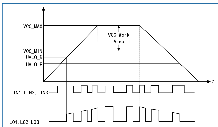
Figure 4-8 Low-side Power Supply VCC and Under-voltage Lockout
