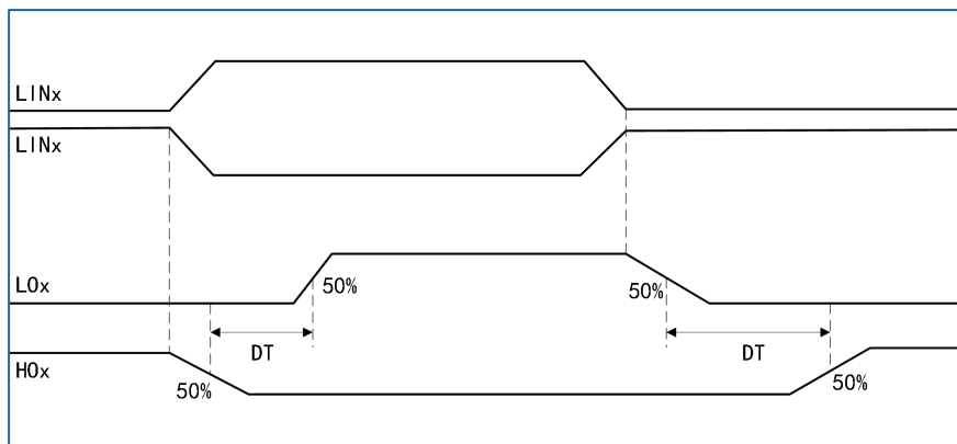
Figure 4-11 Dead Time
