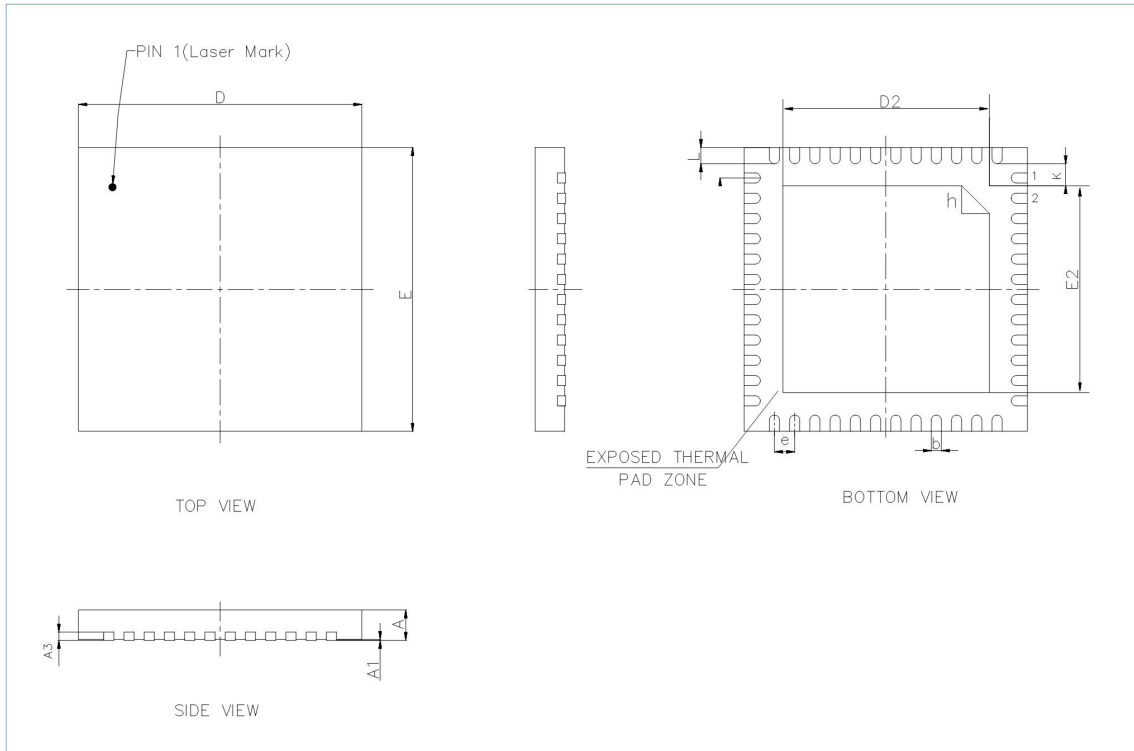
Figure 8-1 WQFN6x6-48 Package Size
