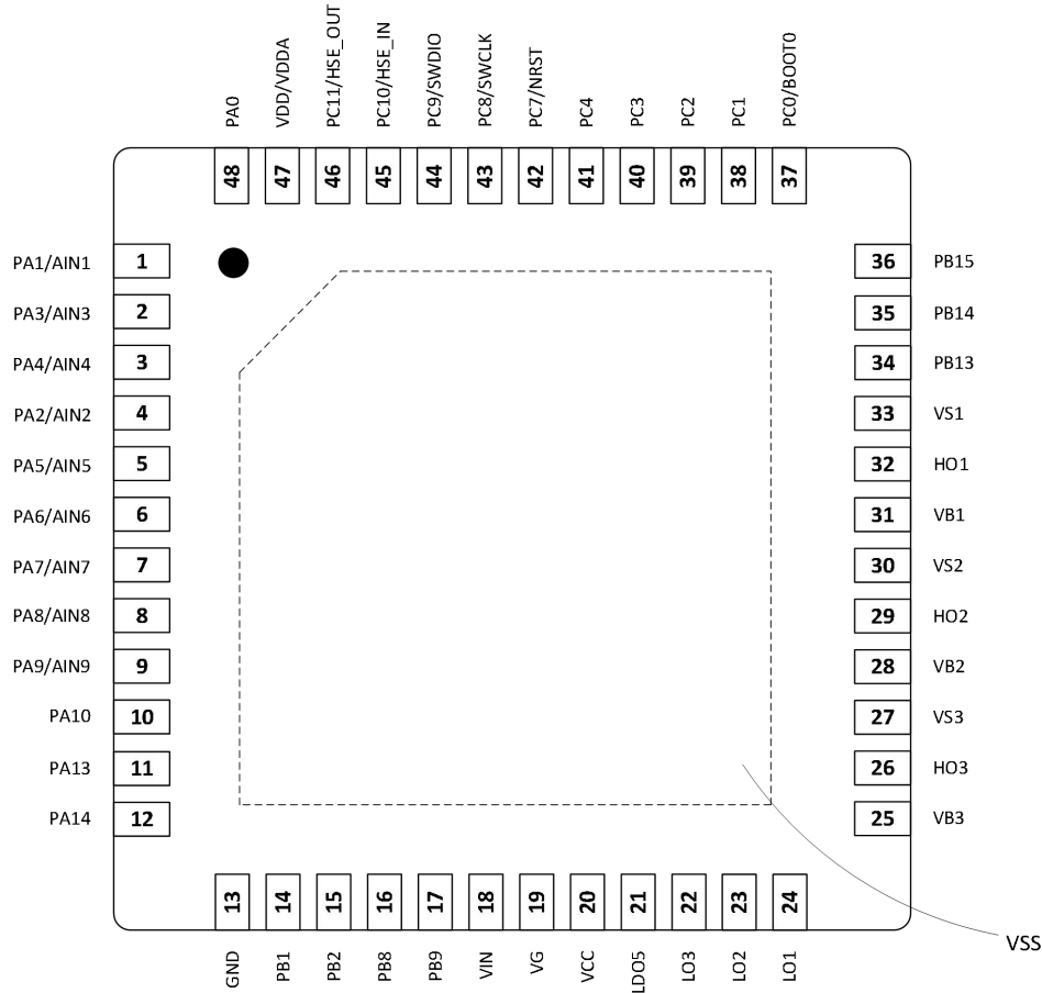
Figure 7-1 Pin Diagram
