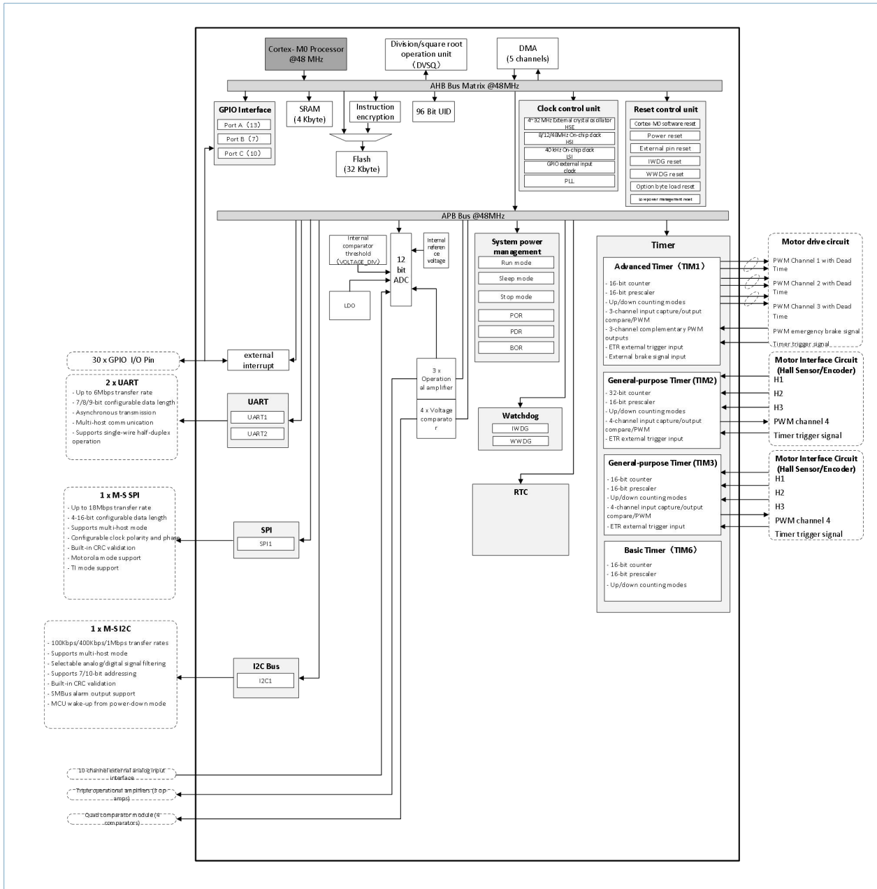
Figure 4-2 PM20025G-08 Functional Block Diagram
