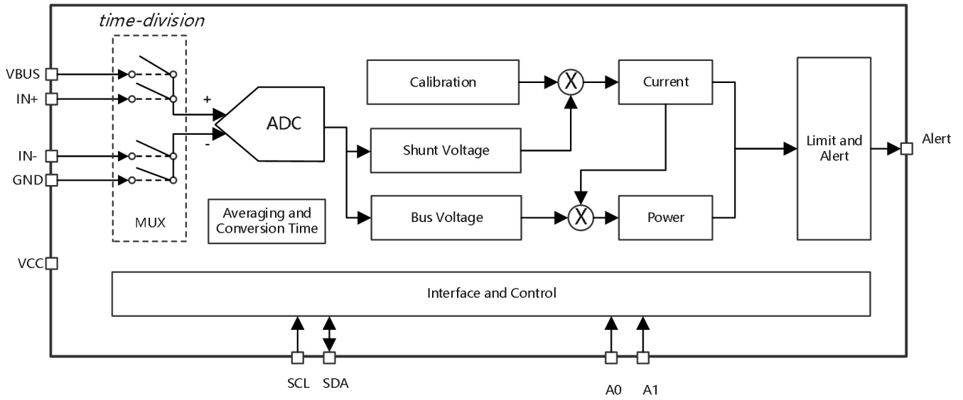
Figure 1-2 Function Block Diagram
