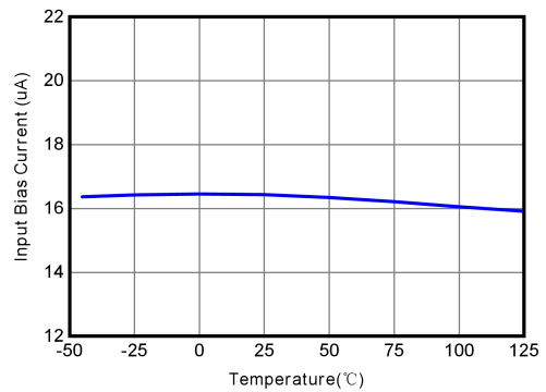
Figure 7-4 Input Bias Current vs Temperature
