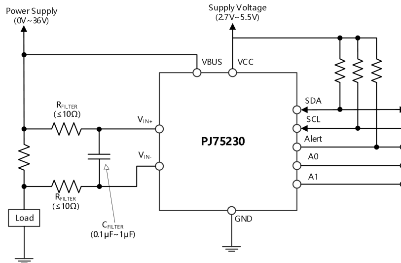
Figure 8-1 Input Filter Circuit
