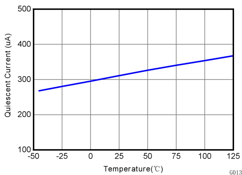
Figure 7-5 Active IQ vs Temperature
