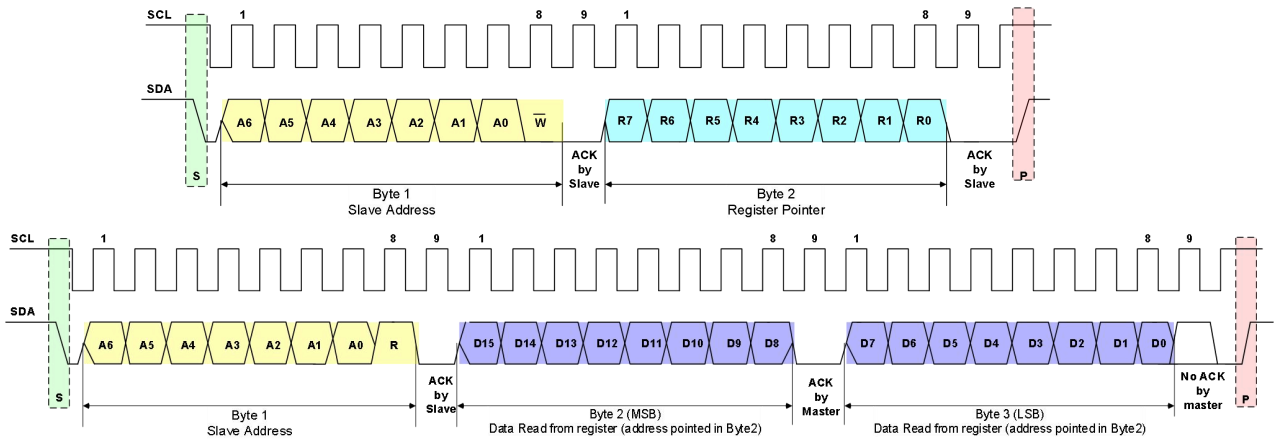
Figure 8-3 Timing Diagram for Read Word Format
