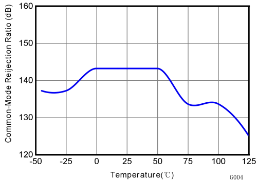
Figure 7-3 Shunt Input CMRR vs Temperature
