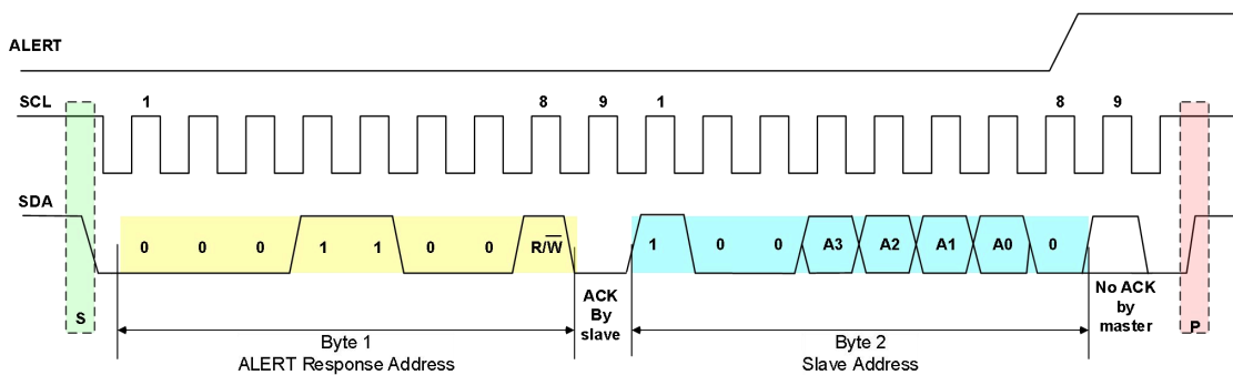
Figure 8-4 Timing Diagram for SMBus ALERT
