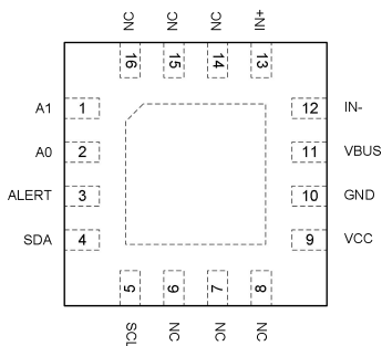
QFN3X3-16
