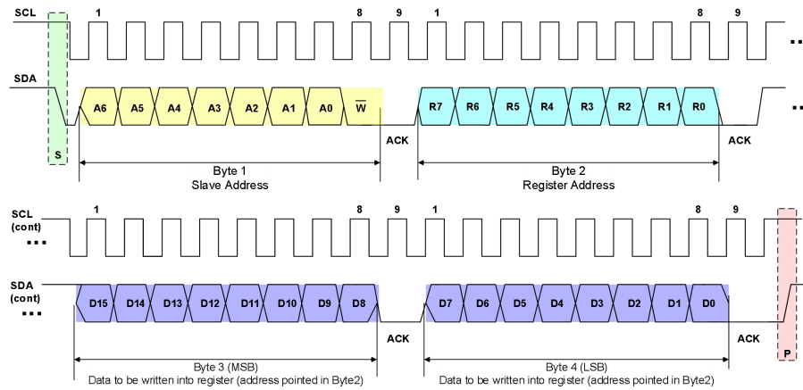
Figure 8-2 Timing Diagram for Write Word Format
