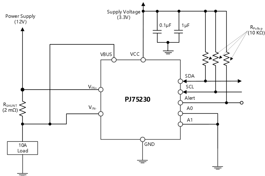
Figure 1-1 Typical Application of PJ75230
