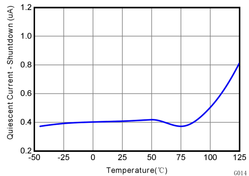
Figure 7-6 Shutdown IQ vs Temperature
