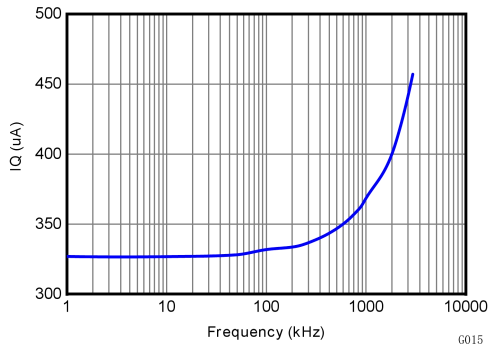
Figure 7-8 Active IQ vs I 2 C Clock Frequency
