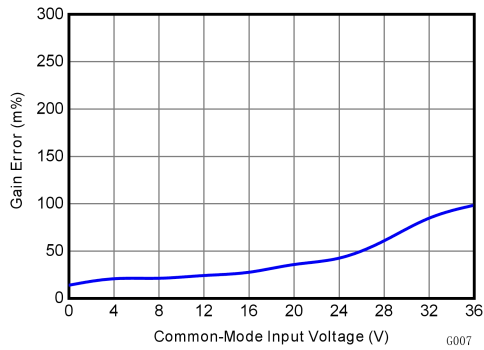
Figure 7-1 Shunt Input Gain Error vs Common-Mode Voltage
