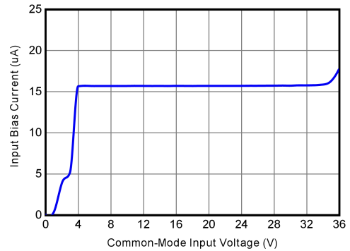
Figure 7-2 Input Bias Current vs Common-Mode Voltage
