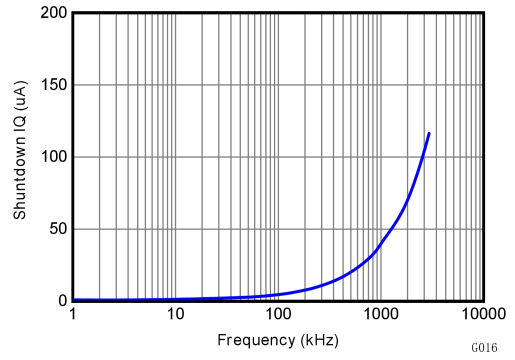
Figure 7-9 Shuttdown IQ vs I 2 C Clock Frequency
