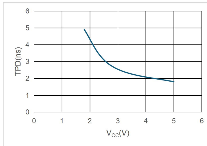
Figure 1. T_{PD} across V_{CC} at 25°C
