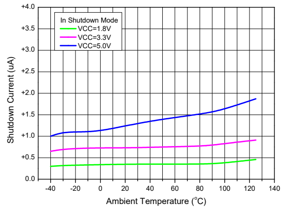
Figure-6. Shutdown Current vs. Temperature
